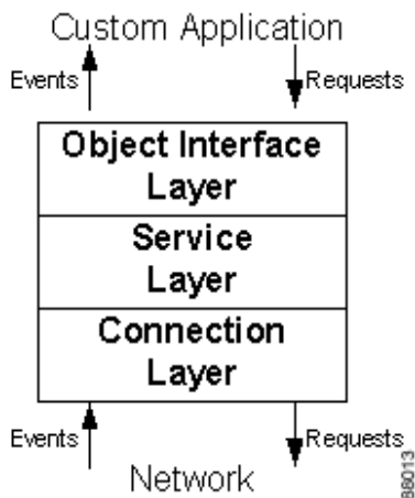
Figure 2-2 Client Interface Library Three-Tiered Architecture
